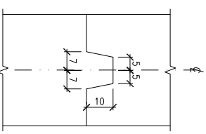
WEB JOINT DETAIL (SCALE 1:1)
