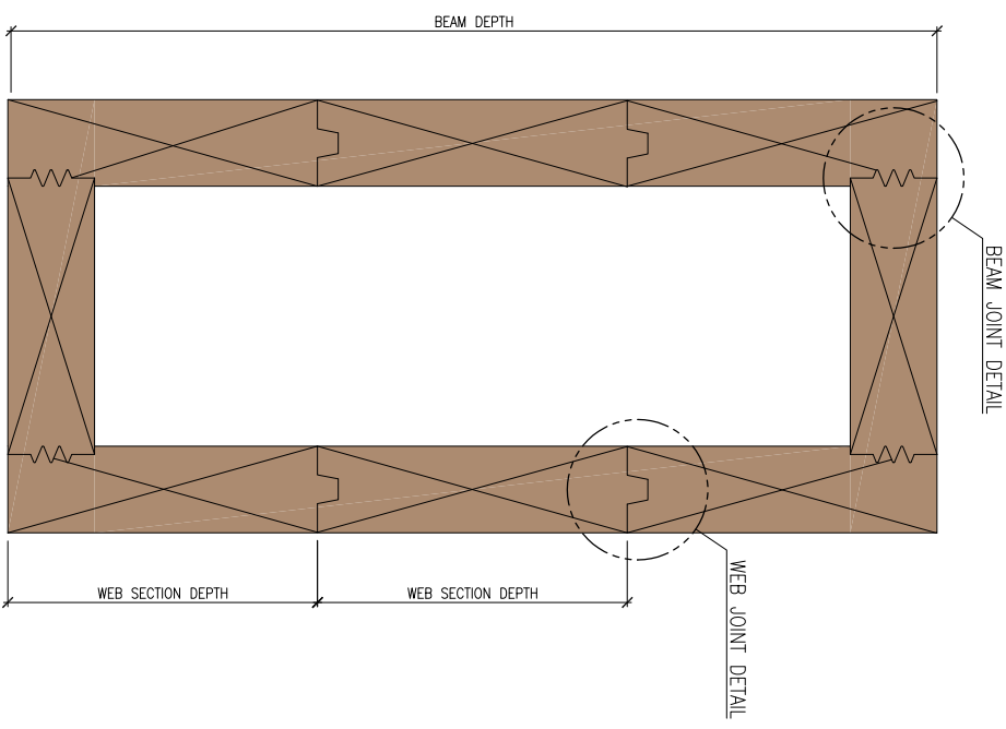
SECTION (SCALE 1:2)
